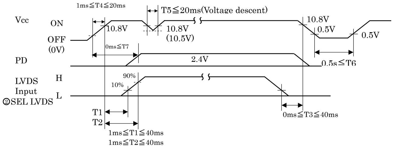
Figure 10-3 Power Supply Sequence (Logic)
