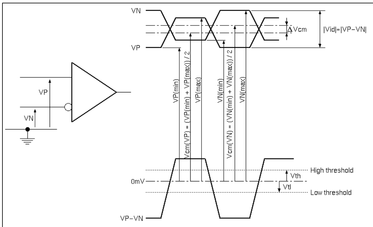
Figure. Voltage Definitions
